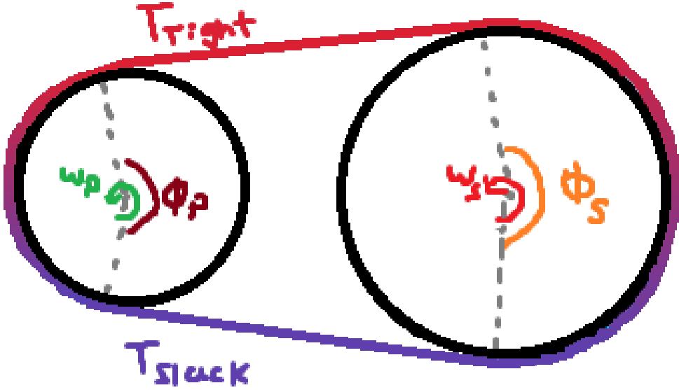
Figure 27: Torque transmission requires a tight–slack tension difference across the wrap.
